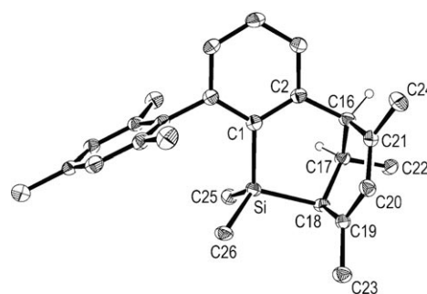
Figure 1. ORTEP of 3 + with ellipsoids set at 30% probability. Hydrogen atoms are omitted for clarity (except for those at C16 and C17).
