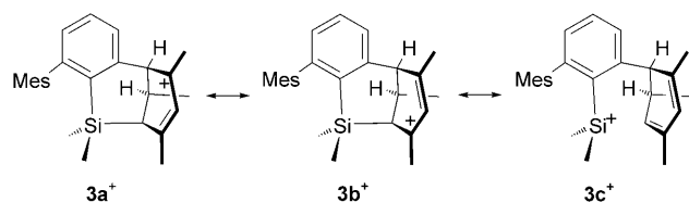
Scheme 4. Principal resonance forms of 3 + .
